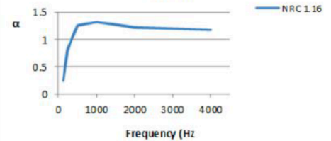
Acoustic Performance 2" Thick Thick
