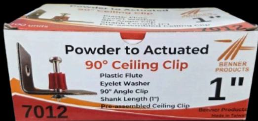
Powder-Driven Pins
